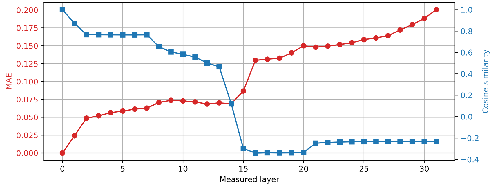
OLMo-7B-hf | Prompt 4 Spared layer 25 | Hybrid vs unquantized
