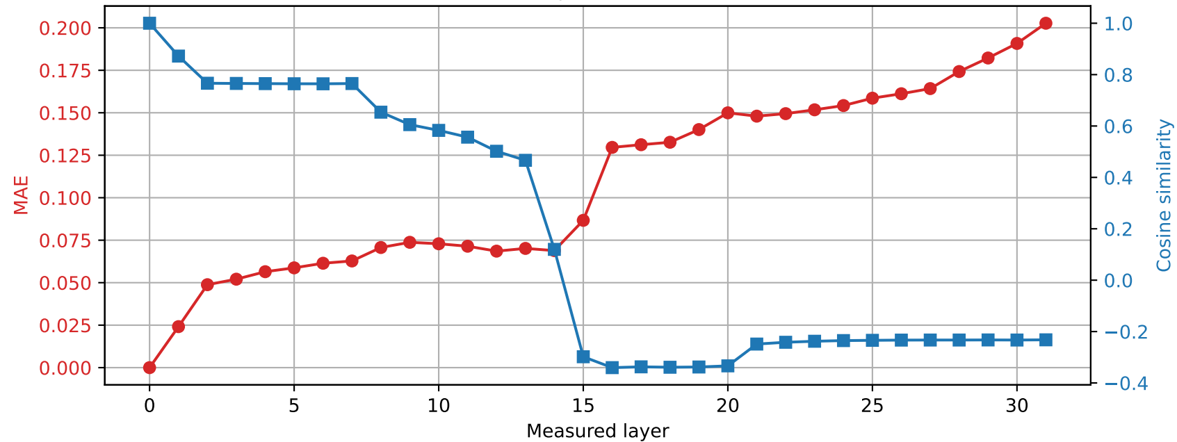
OLMo-7B-hf | Prompt 4 Spared layer 27 | Hybrid vs unquantized
