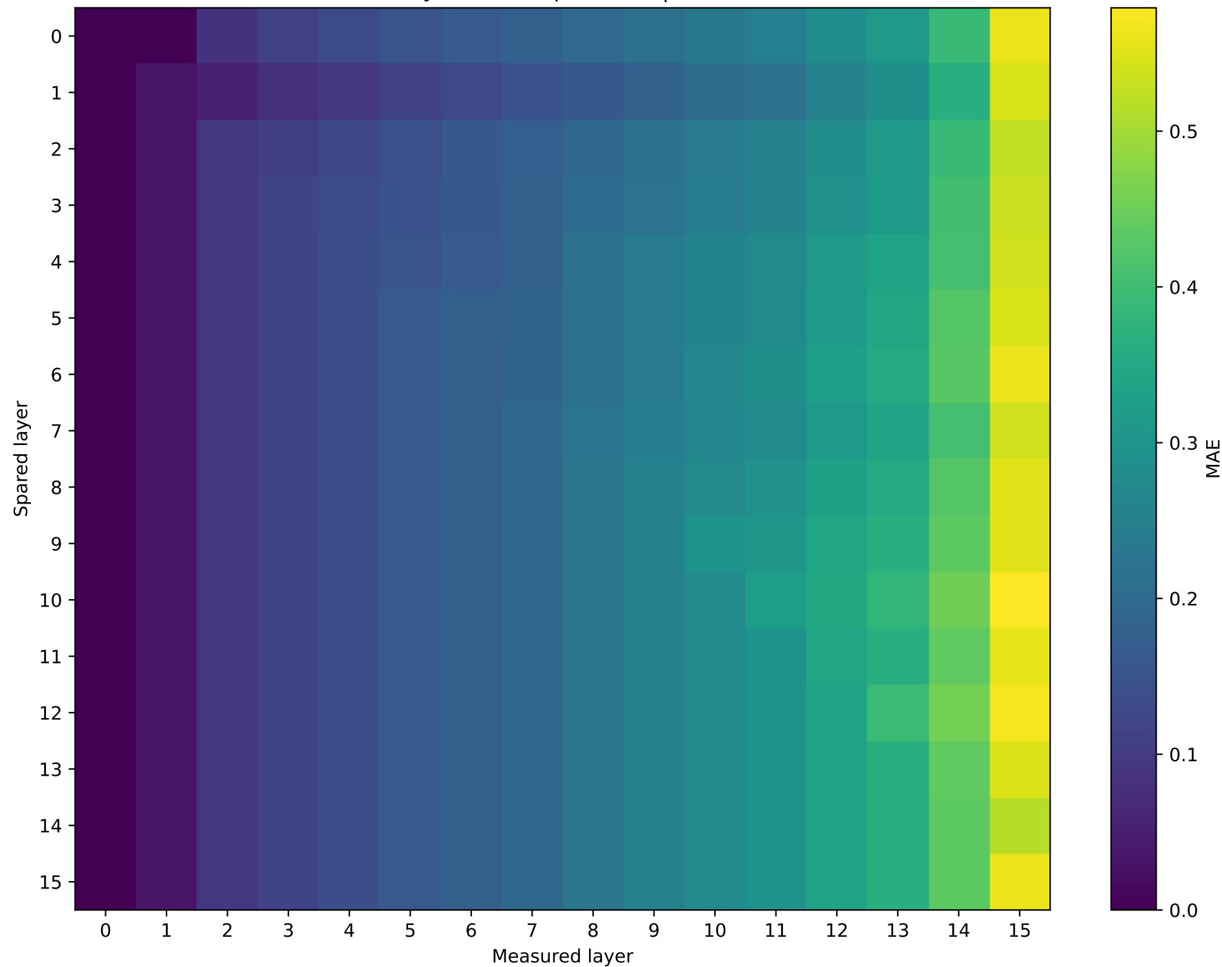
Llama-3.2-1B | Prompt 3 Hybrid vs unquantized | int4
