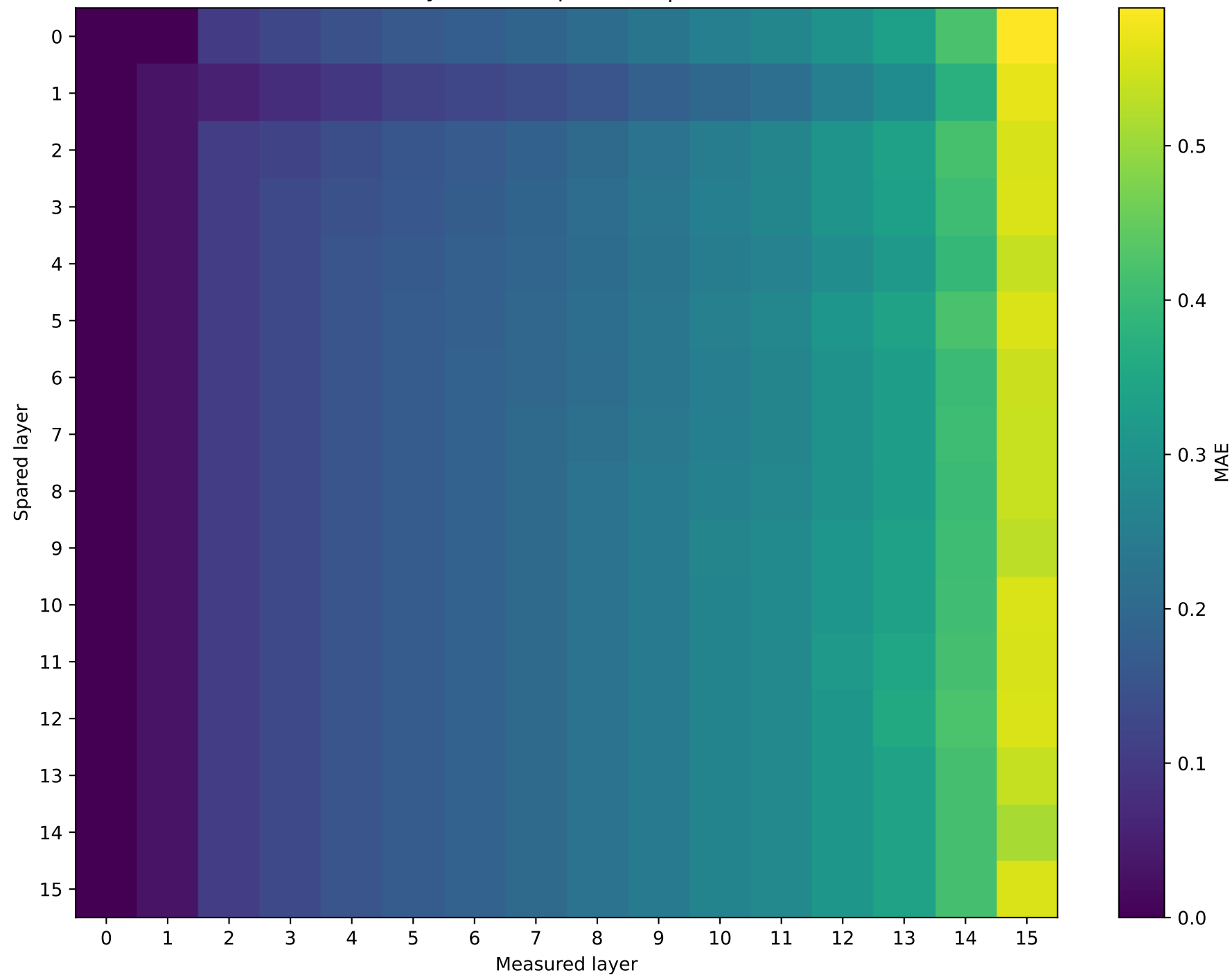
Llama-3.2-1B | Prompt 4 Hybrid vs unquantized | int4
