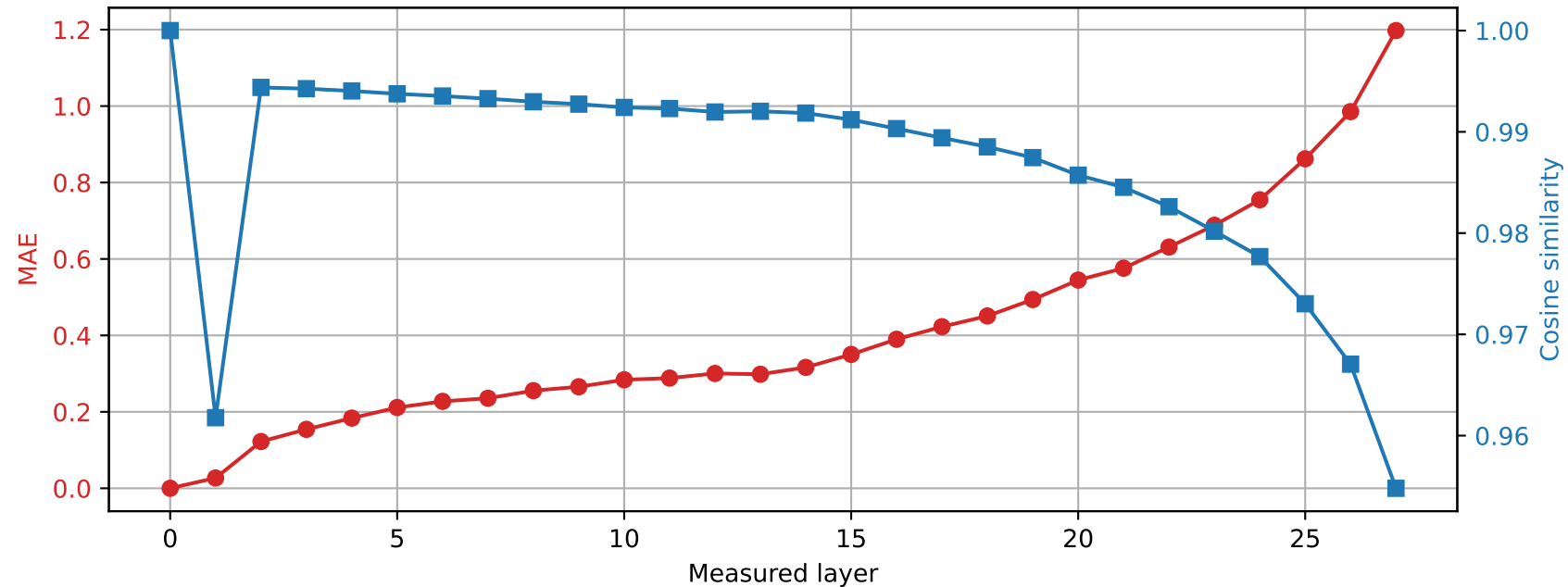
Llama-3.2-3B | Prompt 0 Unquantized vs quantized int4
