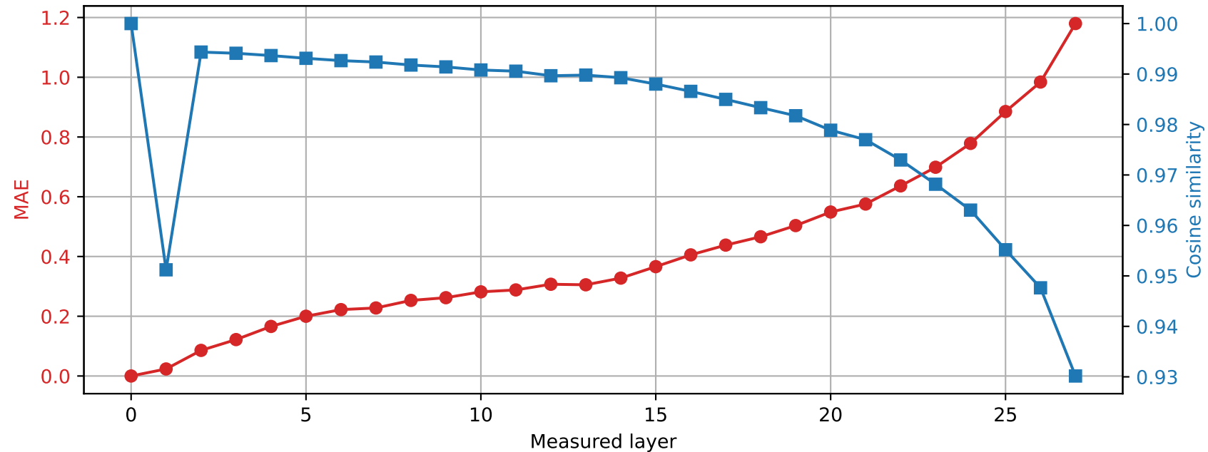
Llama-3.2-3B | Prompt 3 Unquantized vs quantized int4
