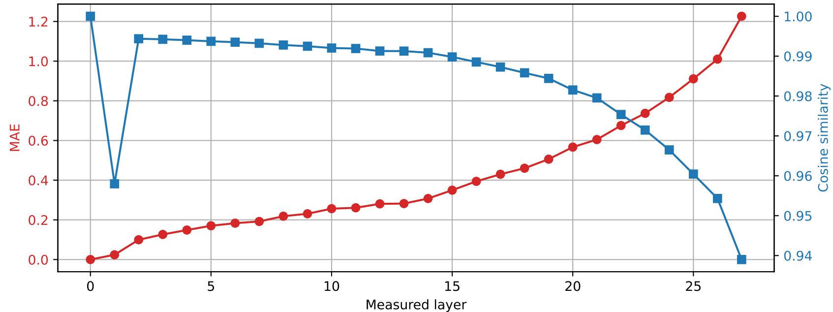
Llama-3.2-3B | Prompt 4 Unquantized vs quantized int4
