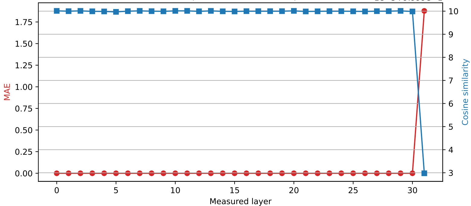
SmolLM2-360M | Quantized layer 30 | float16 \rightarrow int8 1e-5+9.999e-1
