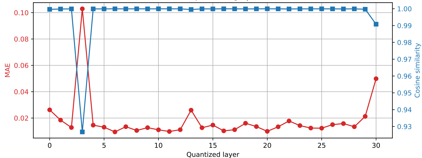
SmolLM2-360M | Prompt 1 Final RMSNorm output damage | float16 \rightarrow int8
