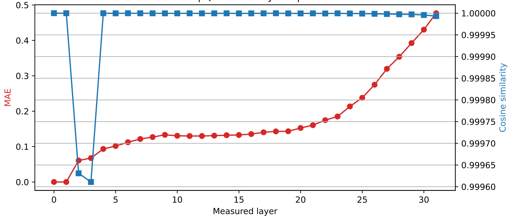
SmolLM2-360M | Quantized layer 1 | float16 \rightarrow int8
