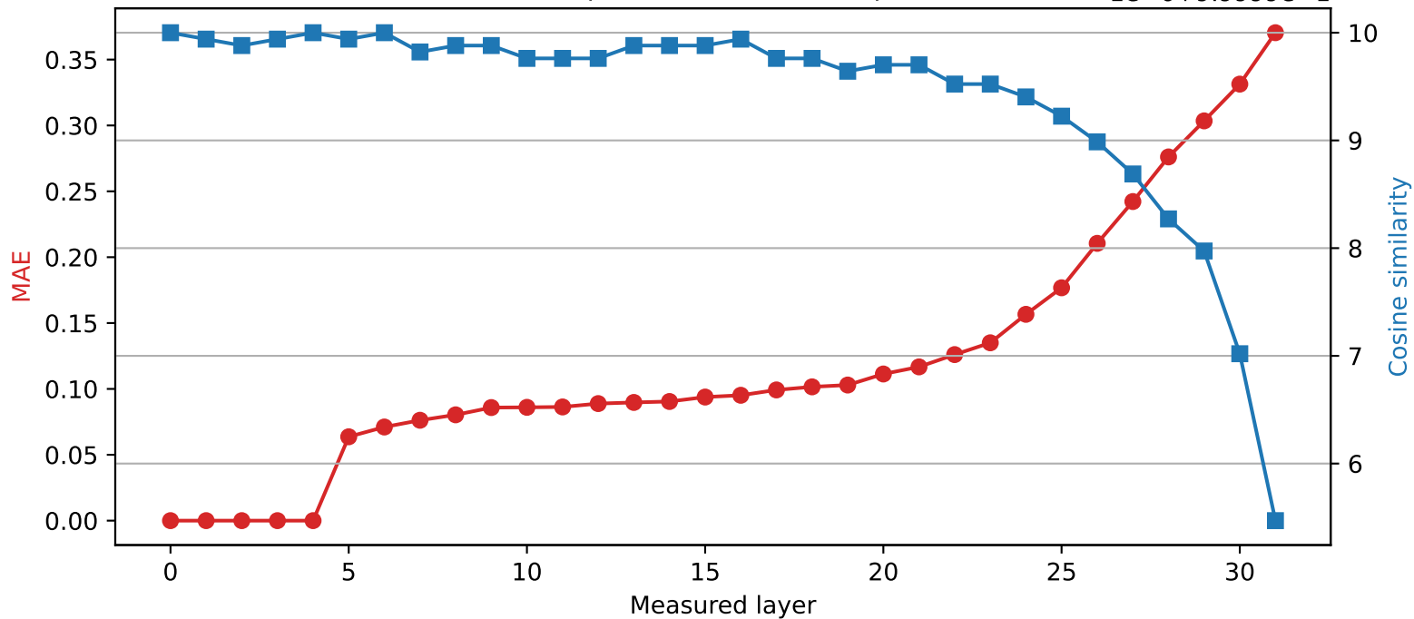
SmolLM2-360M | Quantized layer 4 | float16 → int8 1e-6+9.9999e-1
