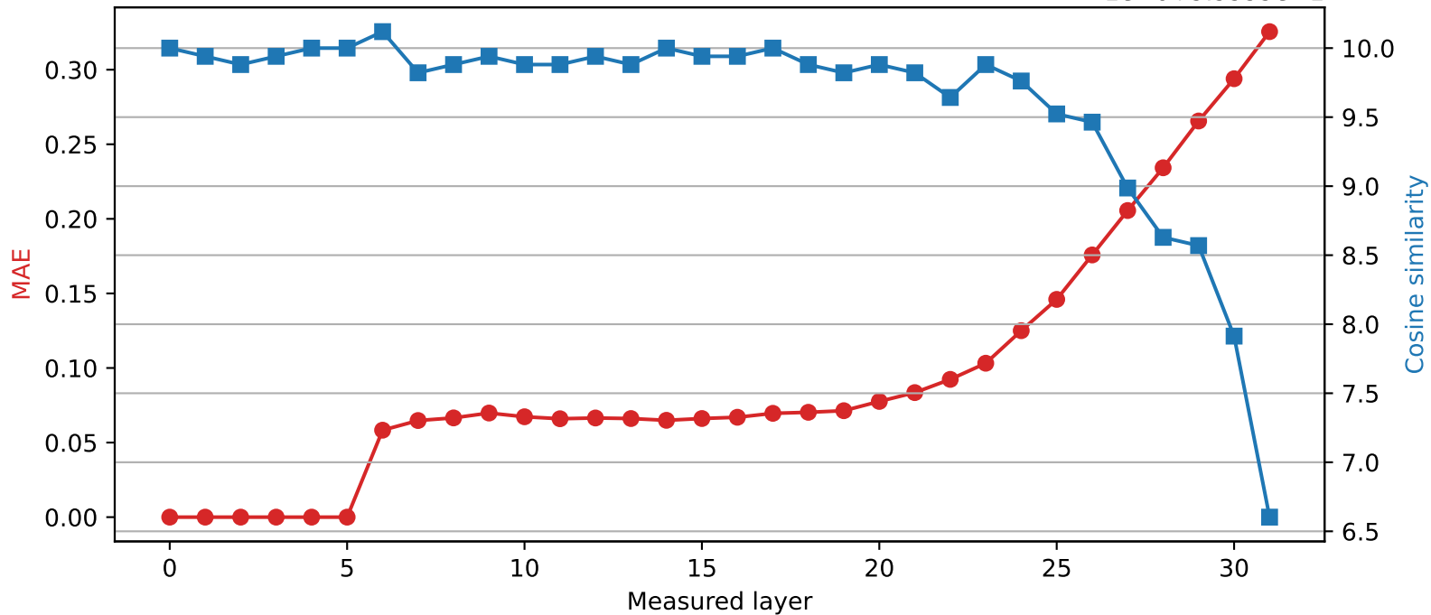
SmolLM2-360M | Quantized layer 5 | float16 \rightarrow int8 1e-6+9.9999e-1
