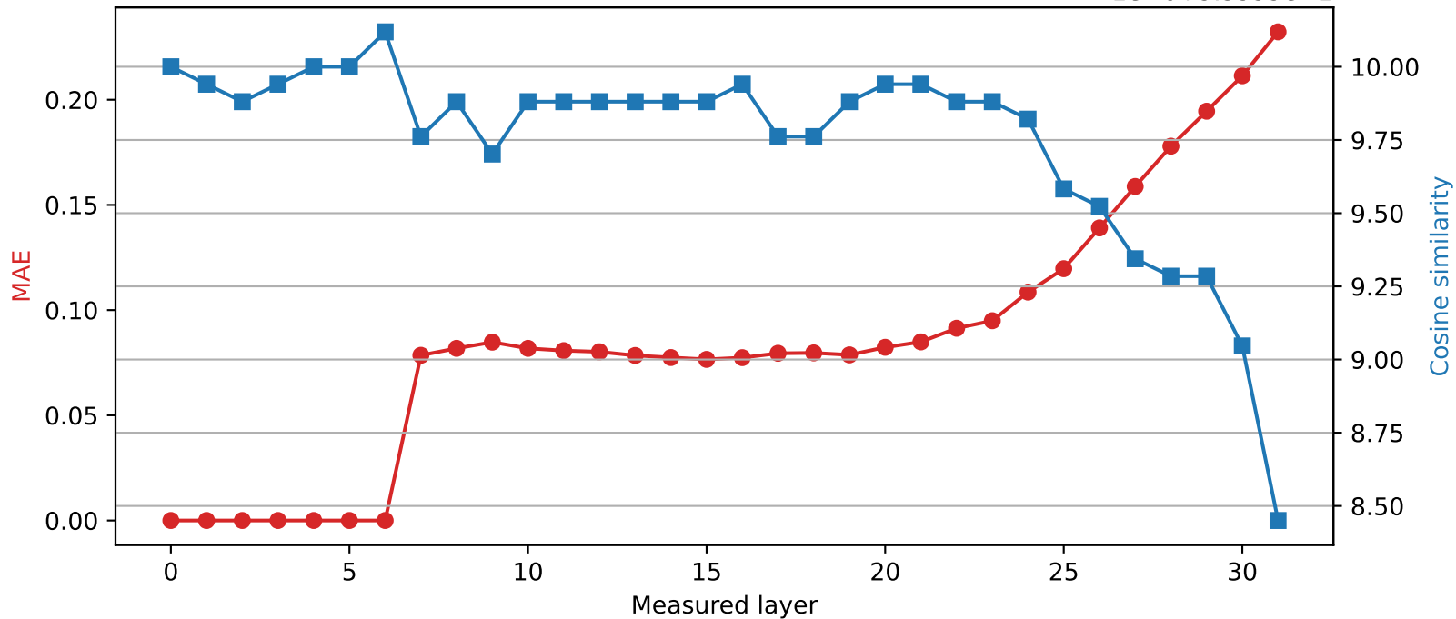
SmolLM2-360M | Quantized layer 6 | float16 \rightarrow int8 1e-6+9.9999e-1
