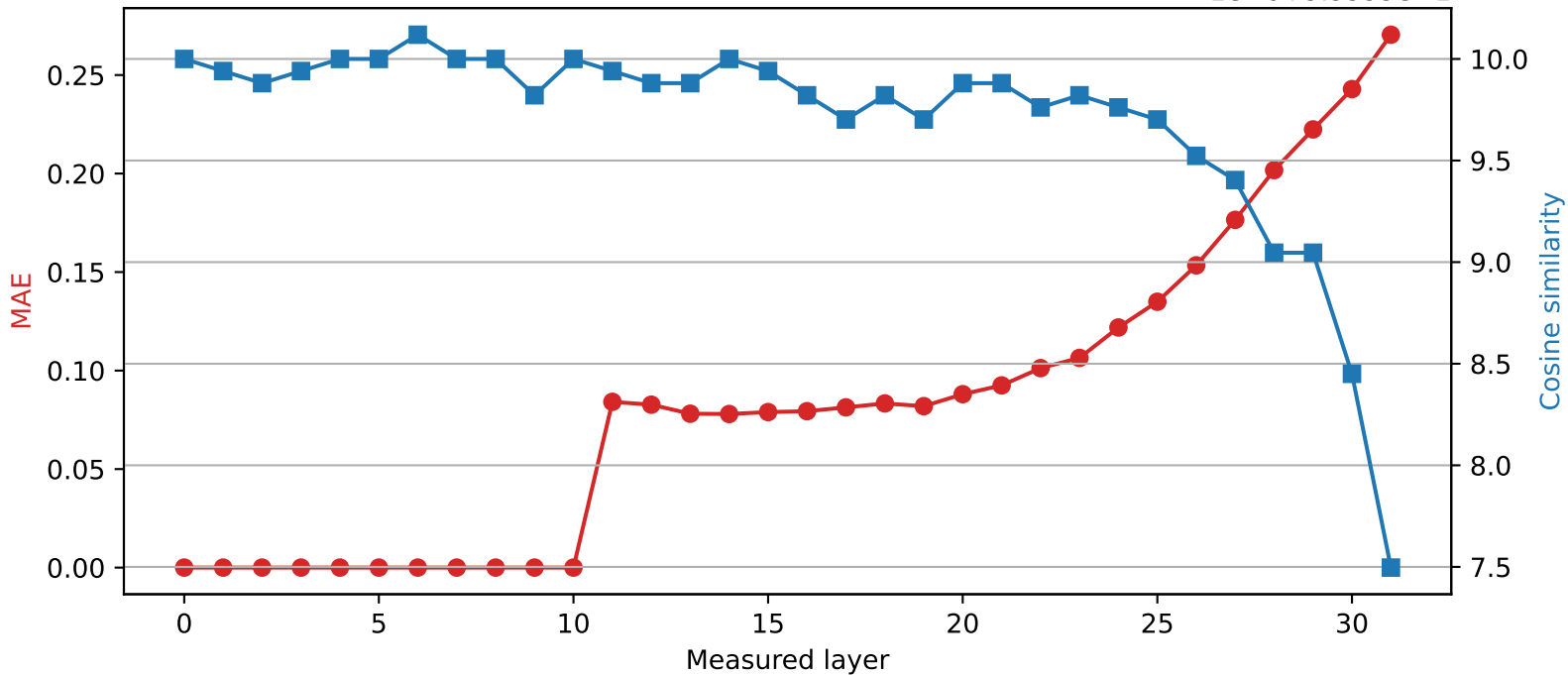
SmolLM2-360M | Quantized layer 10 | float16 \rightarrow int8 1e-6+9.9999e-1
