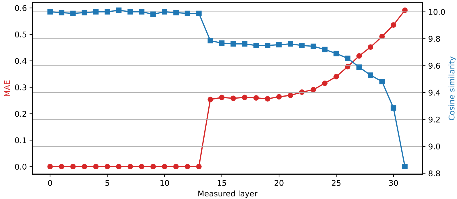
SmolLM2-360M | Quantized layer 13 | float16 → int8 1e-5 + 9.999e-1
