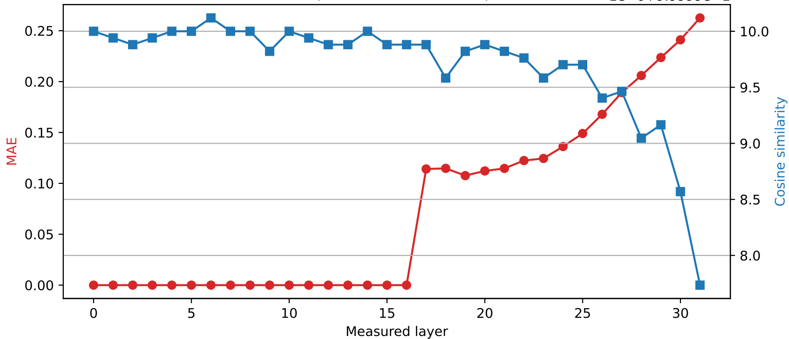
SmolLM2-360M | Quantized layer 16 | float16 \rightarrow int8 1e-6+9.9999e-1
