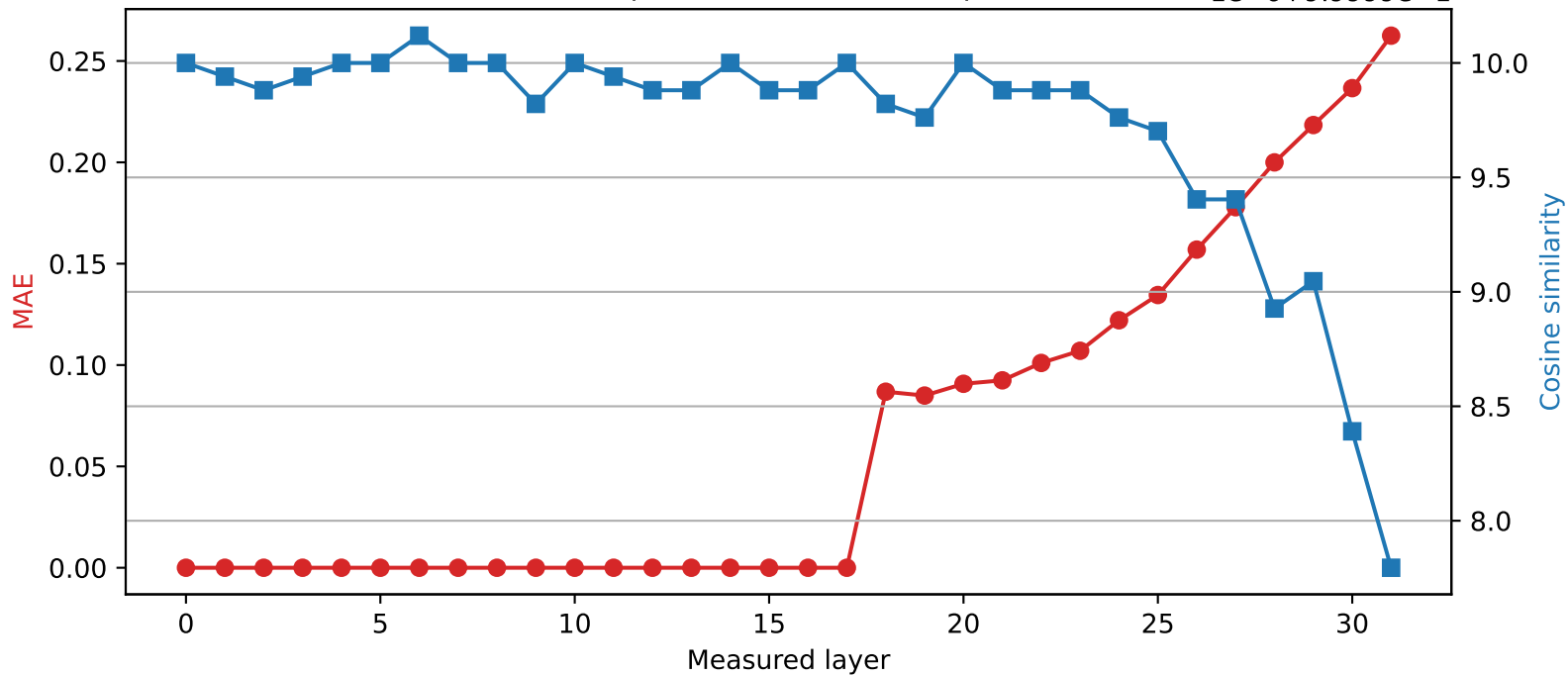
SmolLM2-360M | Quantized layer 17 | float16 \rightarrow int8 1e-6+9.9999e-1
