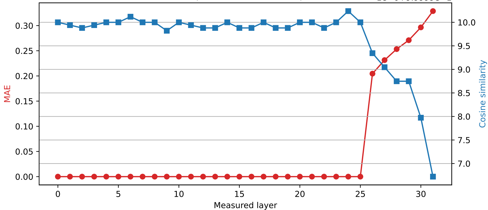
SmolLM2-360M | Quantized layer 25 | float16 \rightarrow int8 1e-6+9.9999e-1
