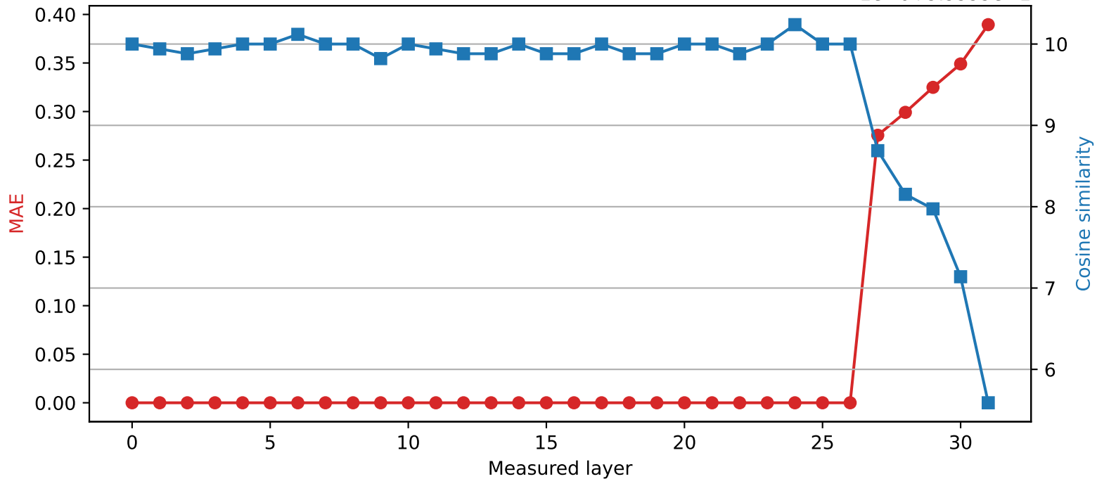
SmolLM2-360M | Quantized layer 26 | float16 \rightarrow int8 1e-6+9.9999e-1
