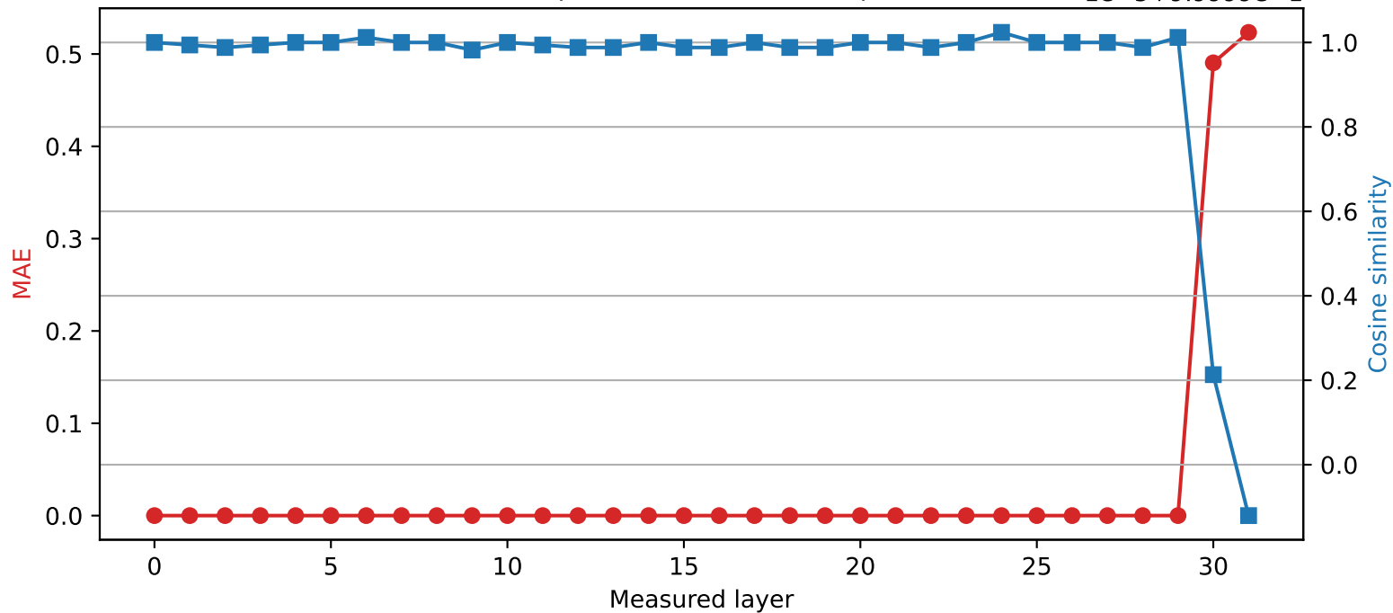
SmolLM2-360M | Quantized layer 29 | float16 \rightarrow int8 1e-5+9.9999e-1
