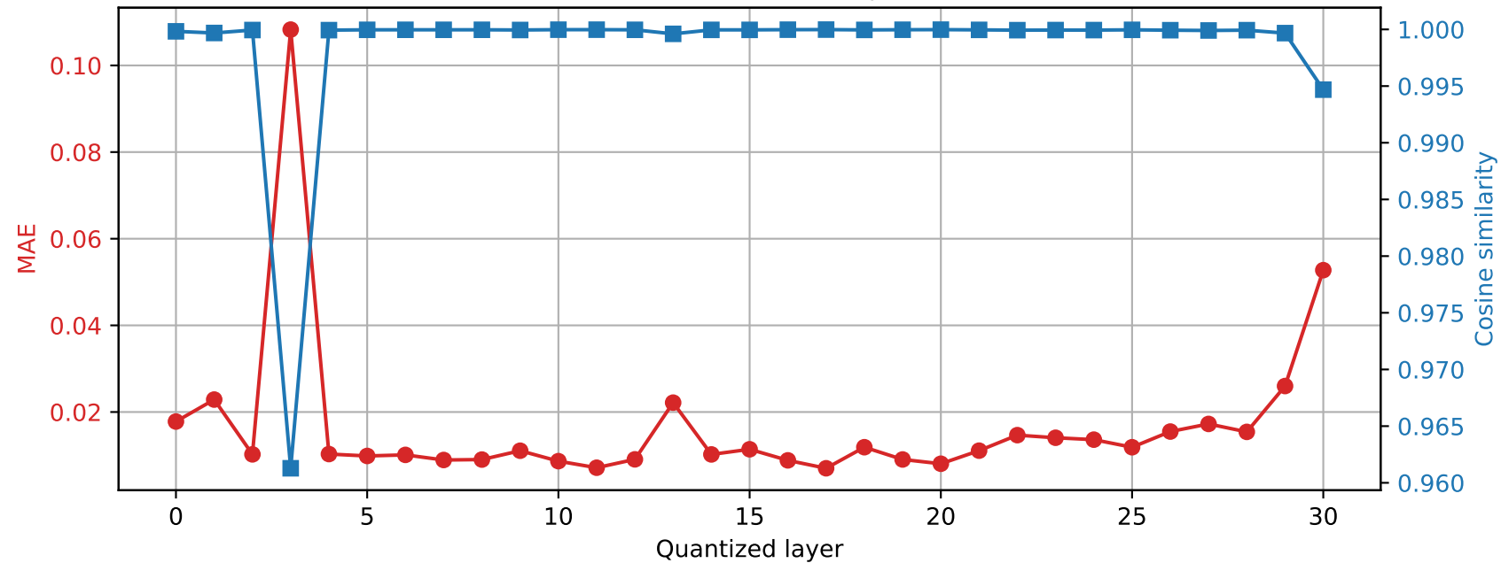
SmolLM2-360M | Prompt 2 Final RMSNorm output damage | float16 → int8
