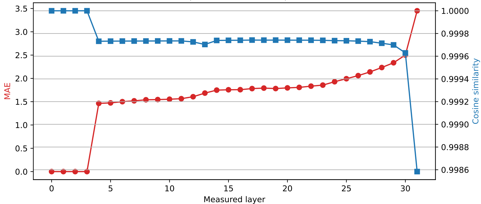
SmolLM2-360M | Quantized layer 3 | float16 \rightarrow int8
