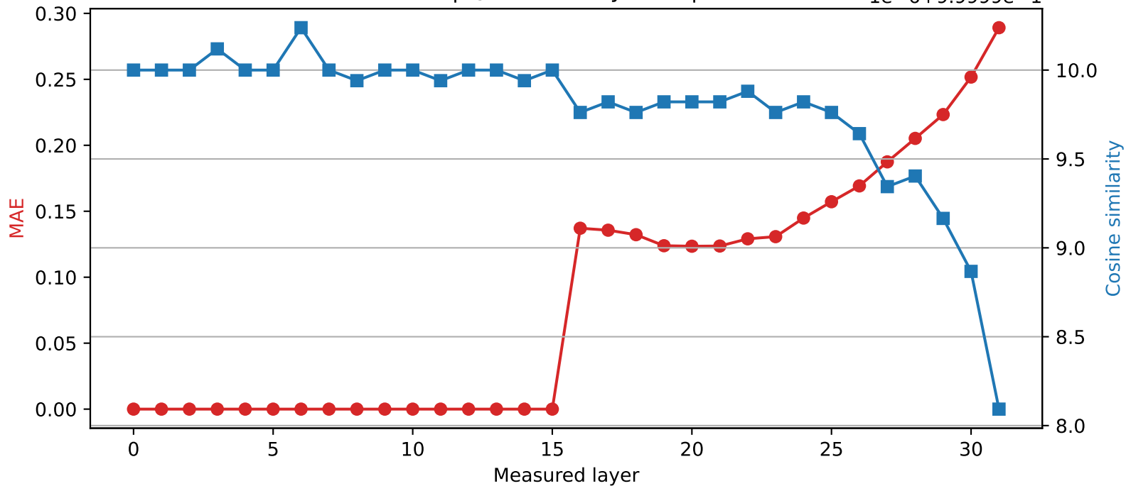
SmolLM2-360M | Quantized layer 15 | float16 \rightarrow int8 1e-6+9.9999e-1
