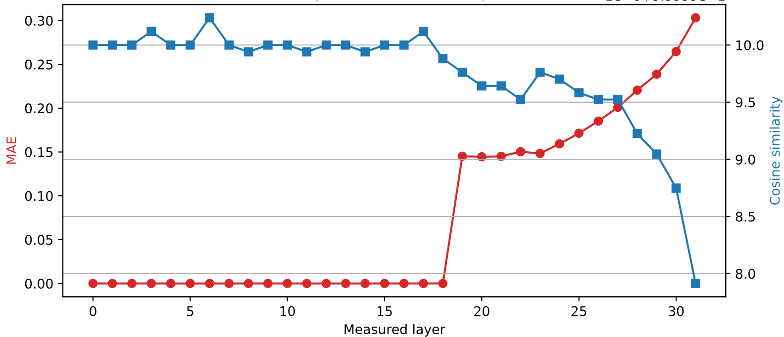
SmolLM2-360M | Quantized layer 18 | float16 \rightarrow int8 1e-6+9.9999e-1
