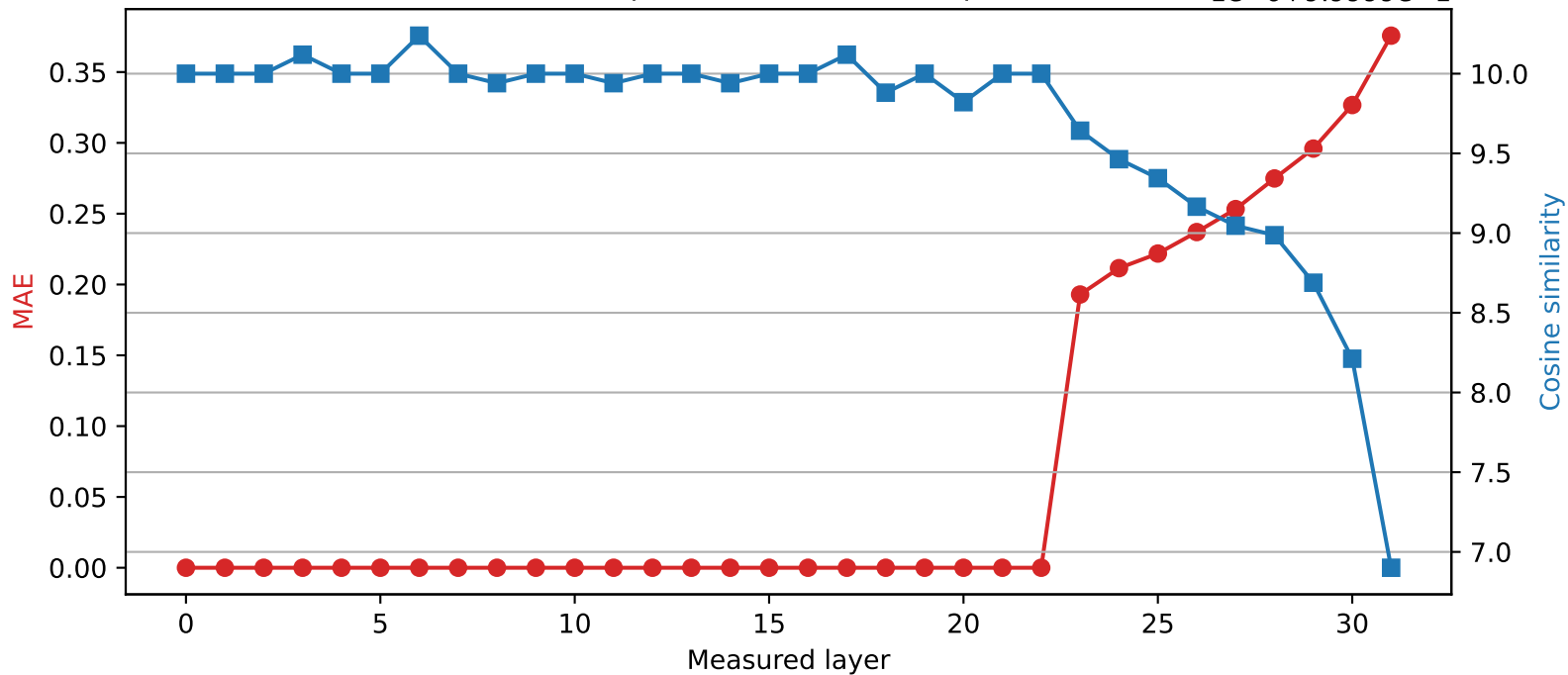
SmolLM2-360M | Quantized layer 22 | float16 \rightarrow int8 1e-6+9.9999e-1
