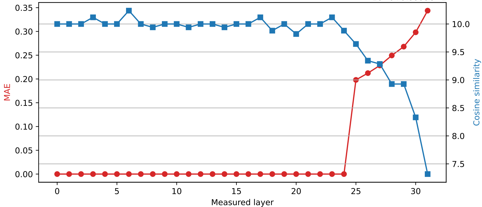
SmolLM2-360M | Quantized layer 24 | float16 \rightarrow int8 1e-6+9.9999e-1
