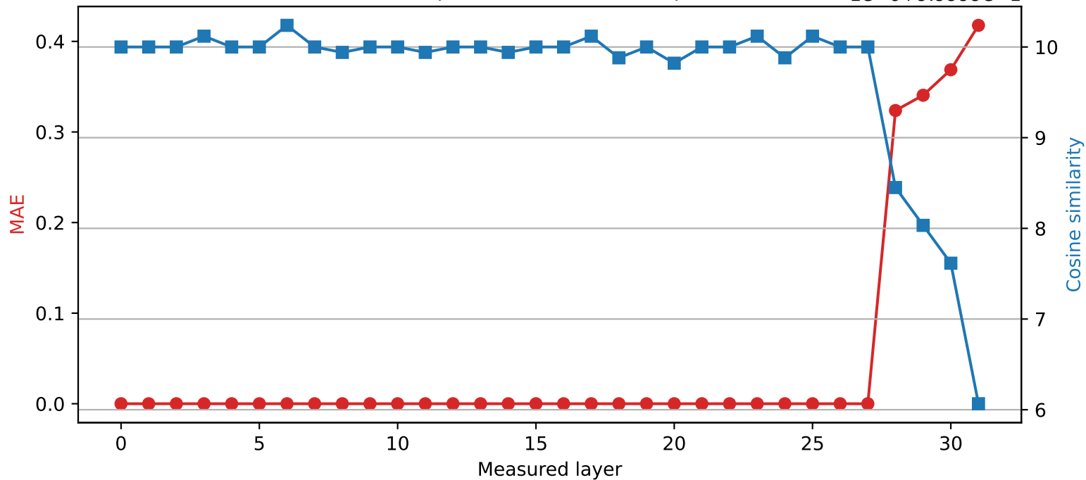
SmolLM2-360M | Quantized layer 27 | float16 \rightarrow int8 1e-6+9.9999e-1
