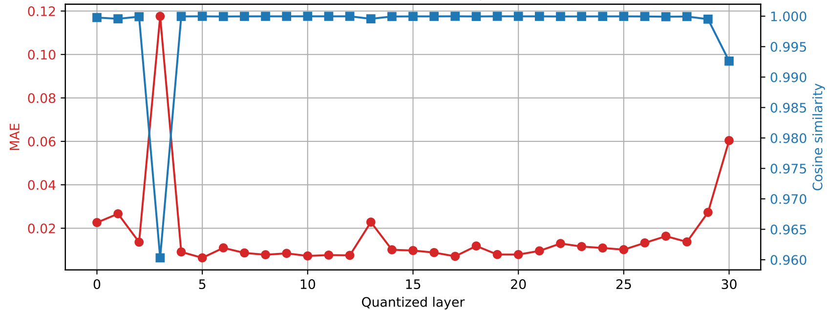
SmolLM2-360M | Prompt 3 Final RMSNorm output damage | float16 \rightarrow int8
