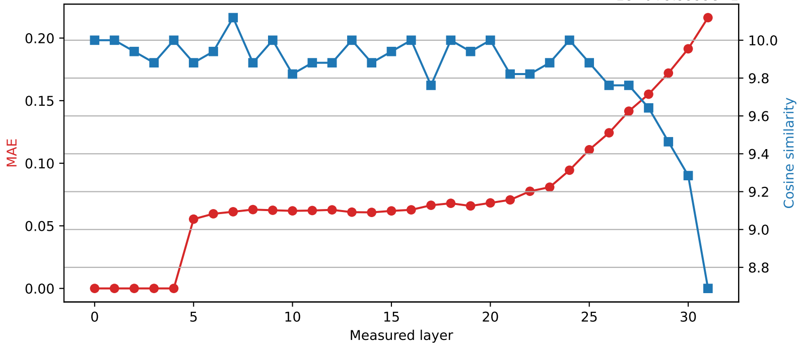
SmolLM2-360M | Quantized layer 4 | float16 \rightarrow int8 1e-6+9.9999e-1
