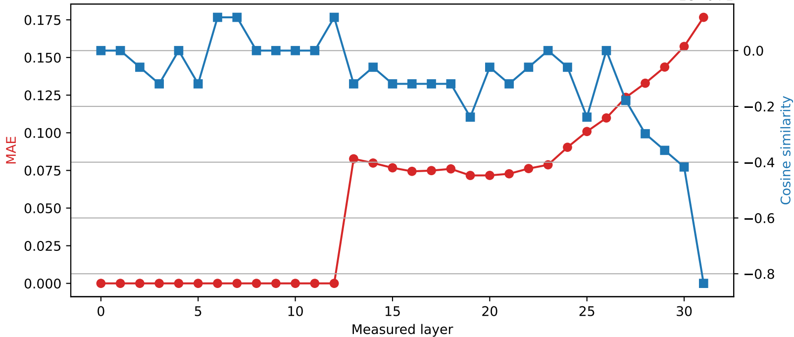
SmolLM2-360M | Quantized layer 12 | float16 → int8
