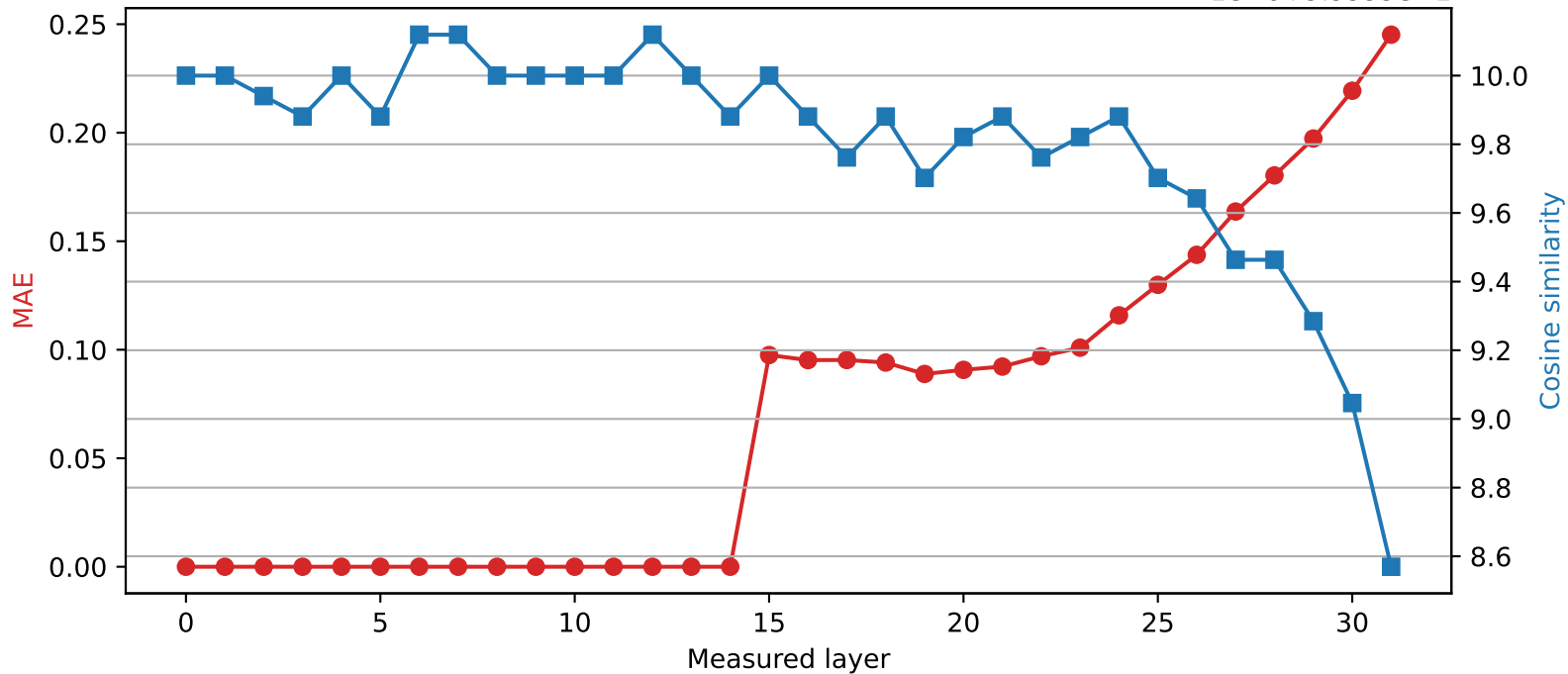
SmolLM2-360M | Quantized layer 14 | float16 \rightarrow int8 1e-6+9.9999e-1
