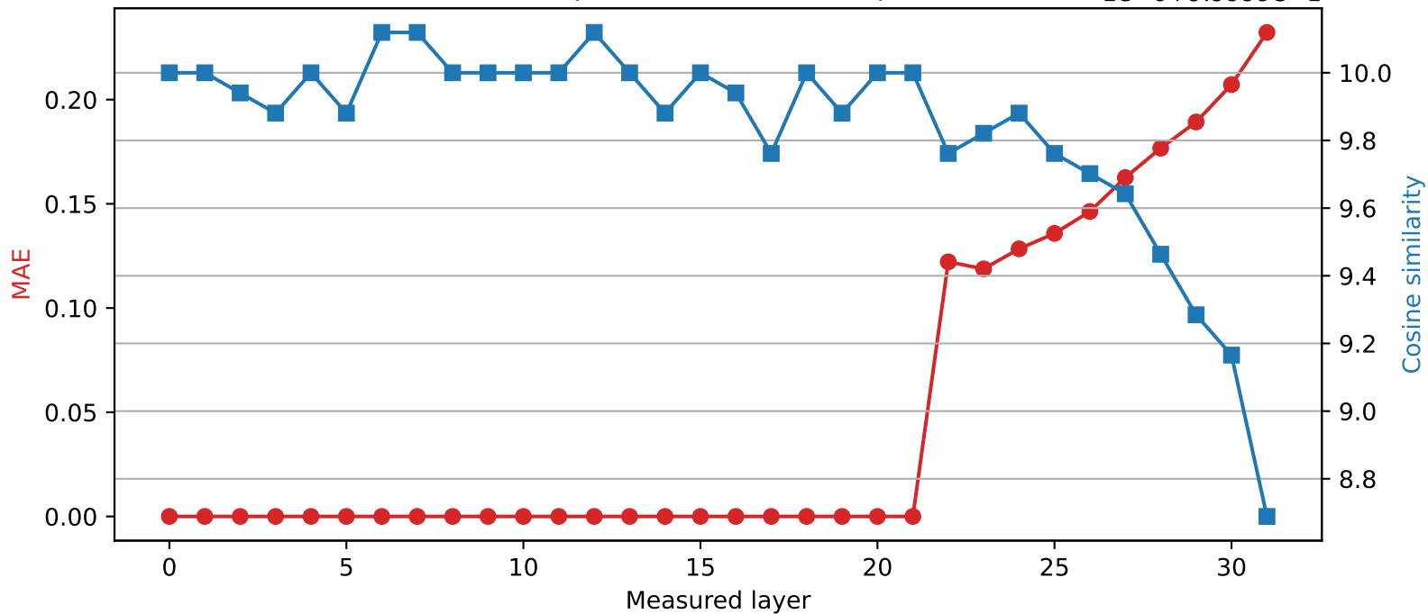
SmolLM2-360M | Quantized layer 21 | float16 \rightarrow int8 1e-6+9.9999e-1
