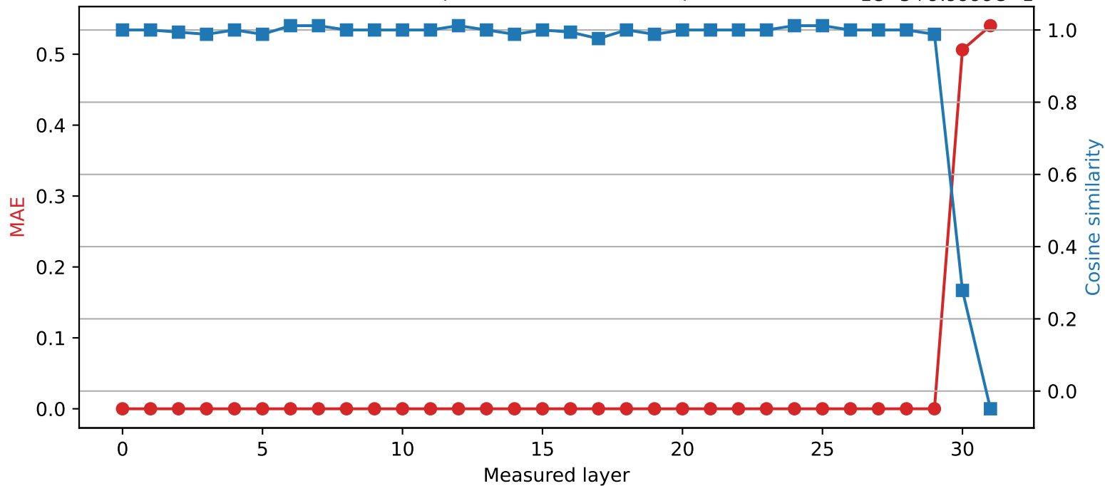
SmolLM2-360M | Quantized layer 29 | float16 \rightarrow int8 1e-5 + 9.9999e-1
