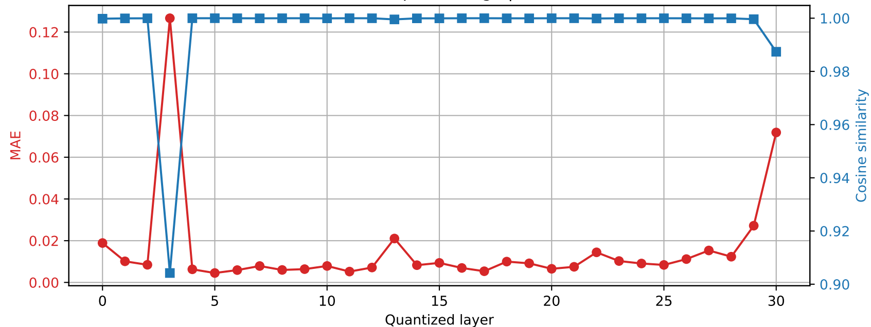
SmolLM2-360M | Prompt 4 Final RMSNorm output damage | float16 \rightarrow int8
