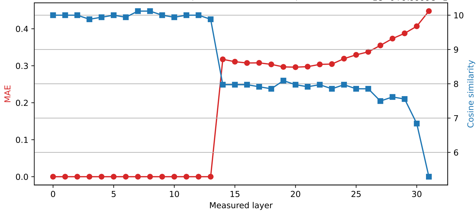
SmolLM2-360M | Quantized layer 13 | float16 \rightarrow int8 1e-6+9.9999e-1
