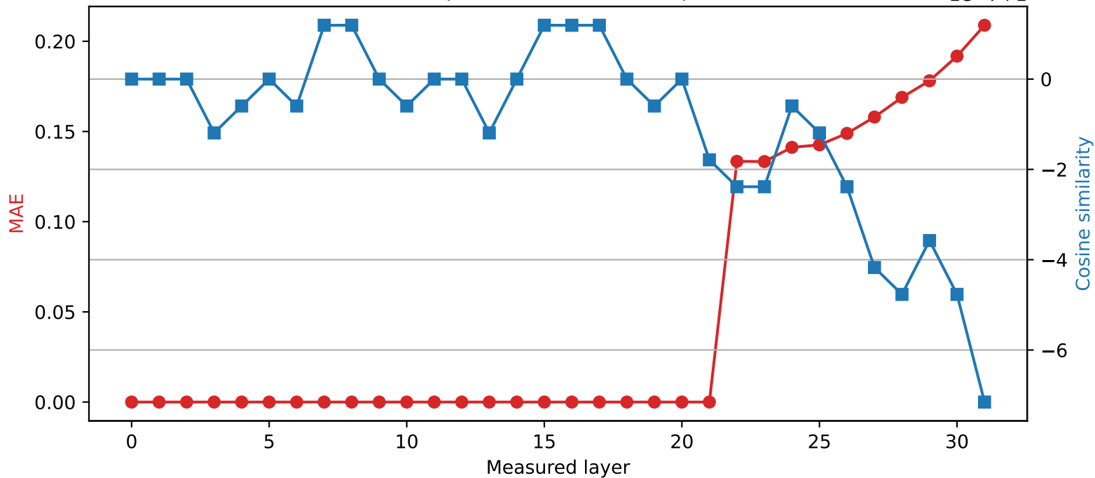
SmolLM2-360M | Quantized layer 21 | float16 \rightarrow int8
