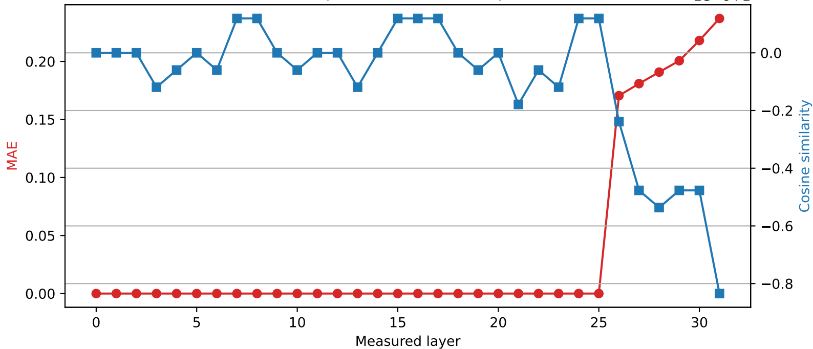
SmolLM2-360M | Quantized layer 25 | float16 → int8
