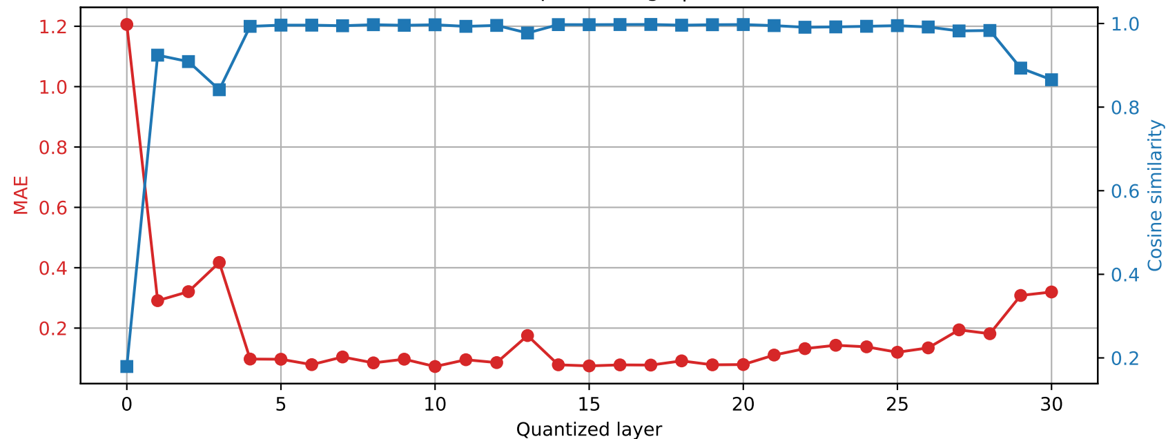
SmolLM2-360M | Prompt 0 Final RMSNorm output damage | float16 → int4
