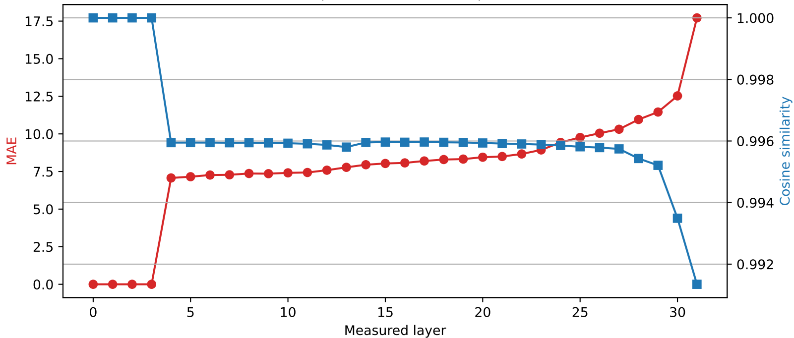
SmolLM2-360M | Quantized layer 3 | float16 \rightarrow int4
