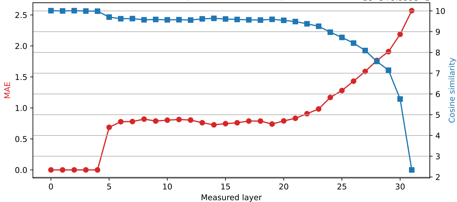
SmolLM2-360M | Quantized layer 4 | float16 → int4
