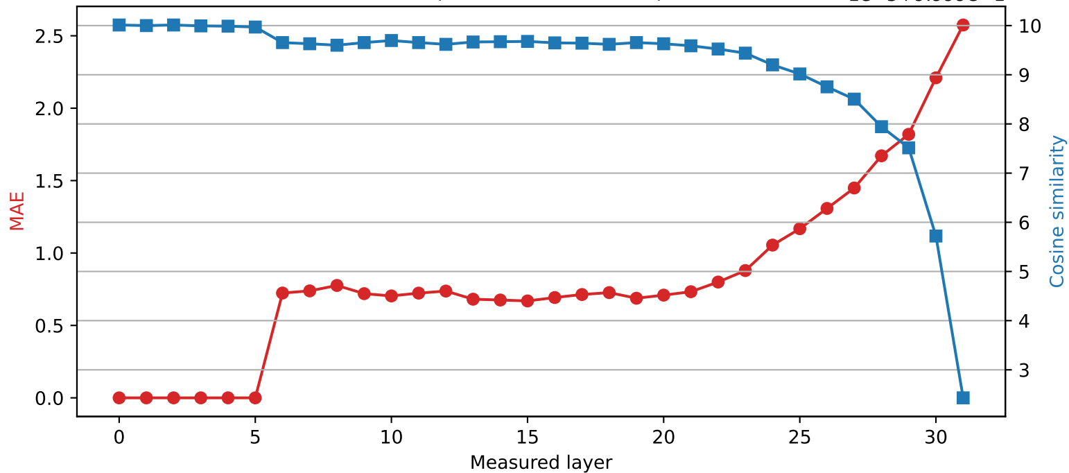
SmolLM2-360M | Quantized layer 5 | float16 → int4
