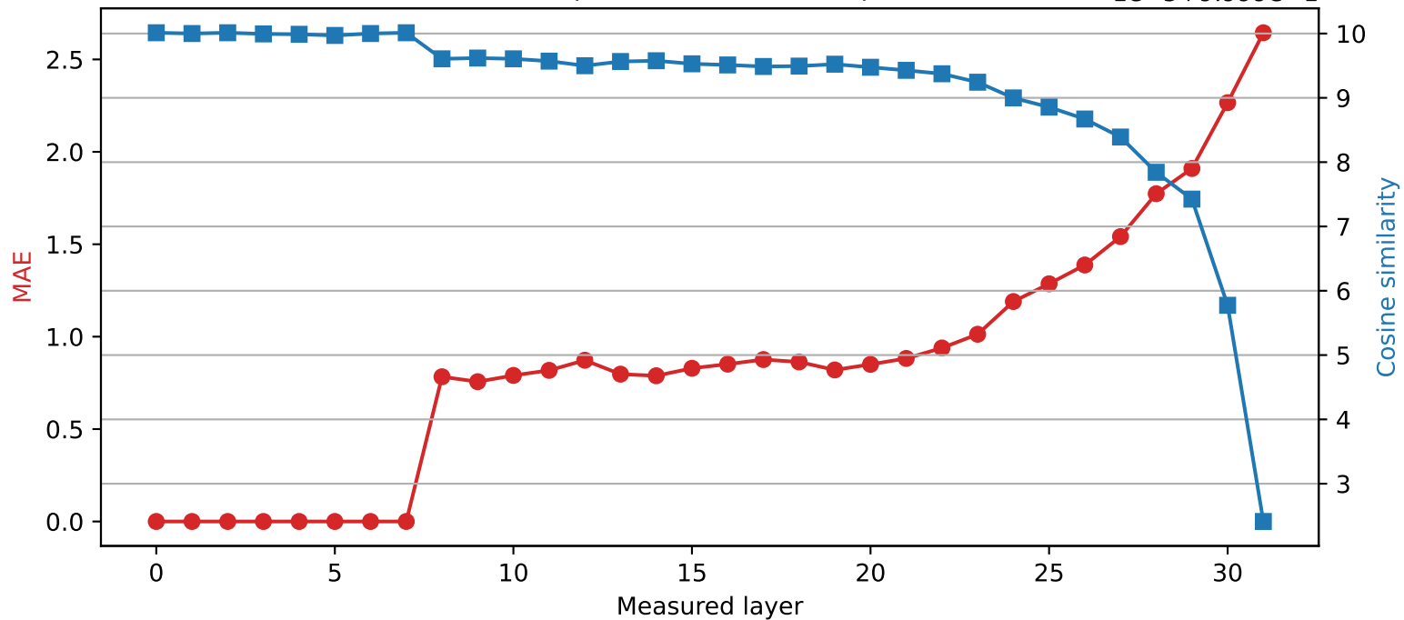
SmolLM2-360M | Quantized layer 7 | float16 → int4
