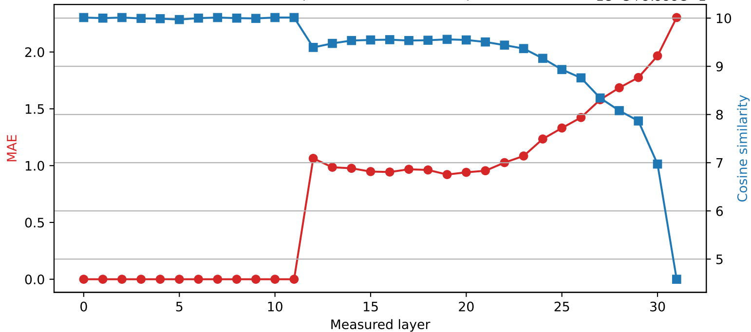
SmolLM2-360M | Quantized layer 11 | float16 → int4 1e-5+9.999e-1
