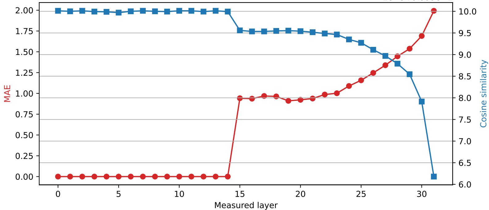
SmolLM2-360M | Quantized layer 14 | float16 → int4 1e-5+9.999e-1
