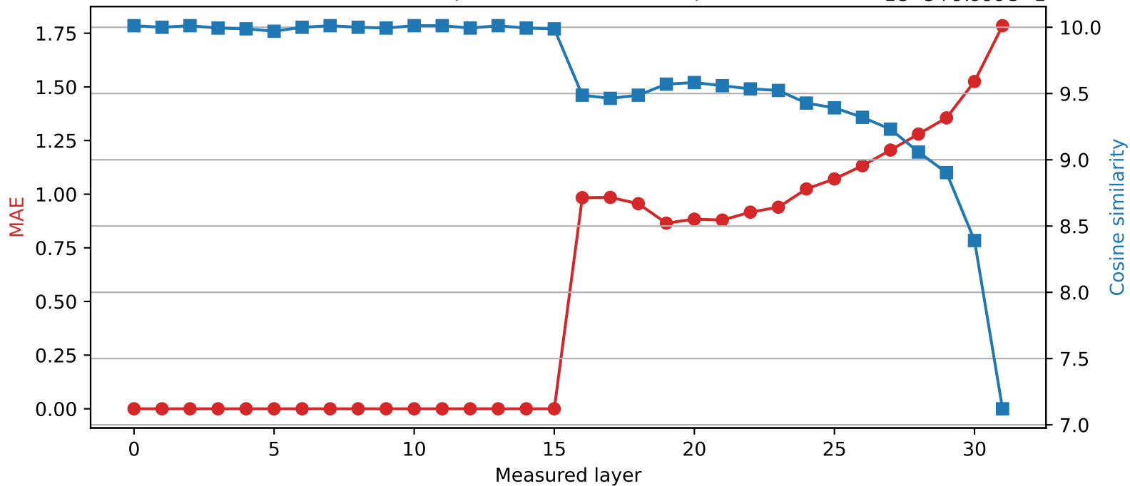
SmolLM2-360M | Quantized layer 15 | float16 \rightarrow int4 1e-5+9.999e-1
