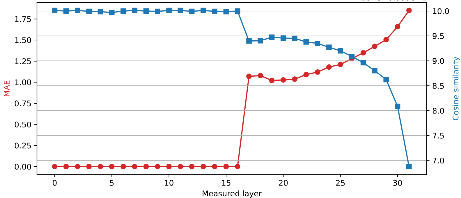
SmolLM2-360M | Quantized layer 16 | float16 \rightarrow int4 1e-5+9.999e-1
