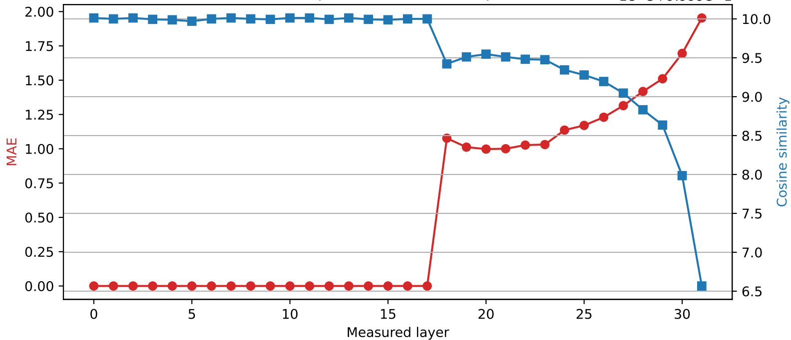
SmolLM2-360M | Quantized layer 17 | float16 \rightarrow int4 1e-5+9.999e-1
