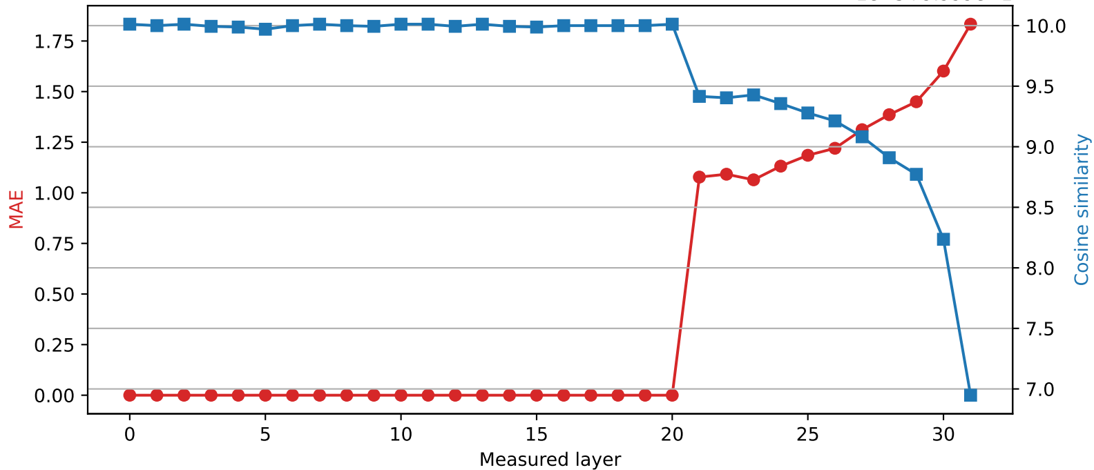
SmolLM2-360M | Quantized layer 20 | float16 \rightarrow int4 1e-5+9.999e-1
