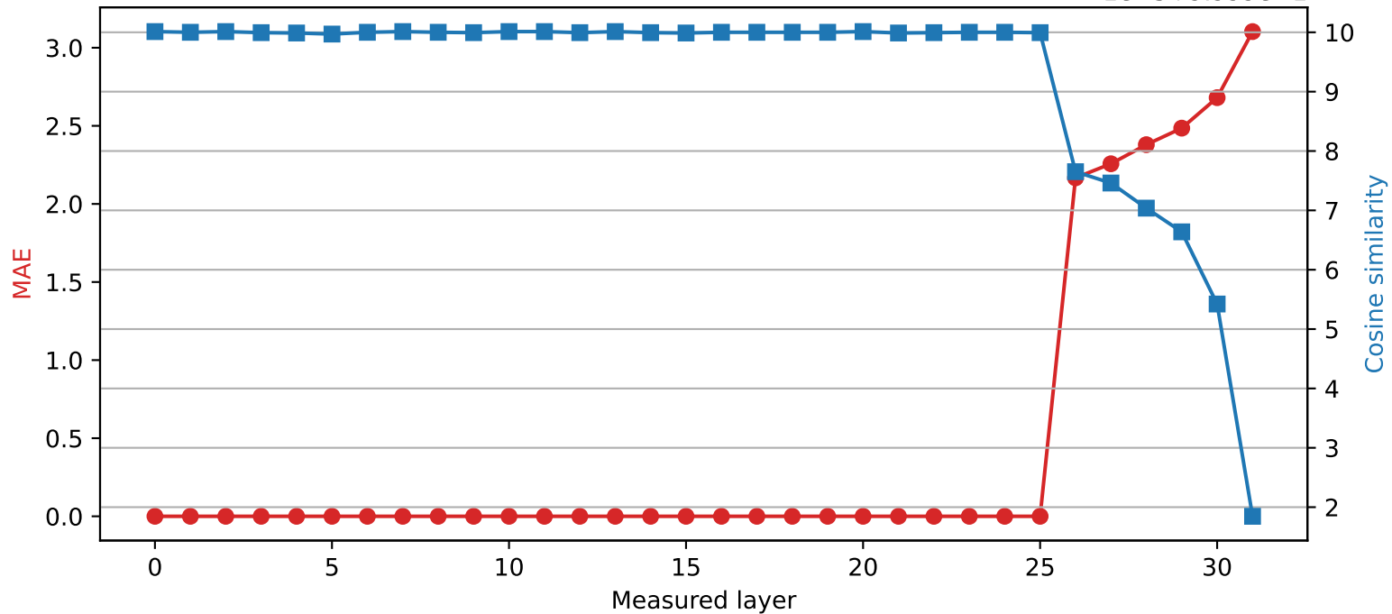
SmolLM2-360M | Quantized layer 25 | float16 \rightarrow int4 1e-5+9.999e-1
