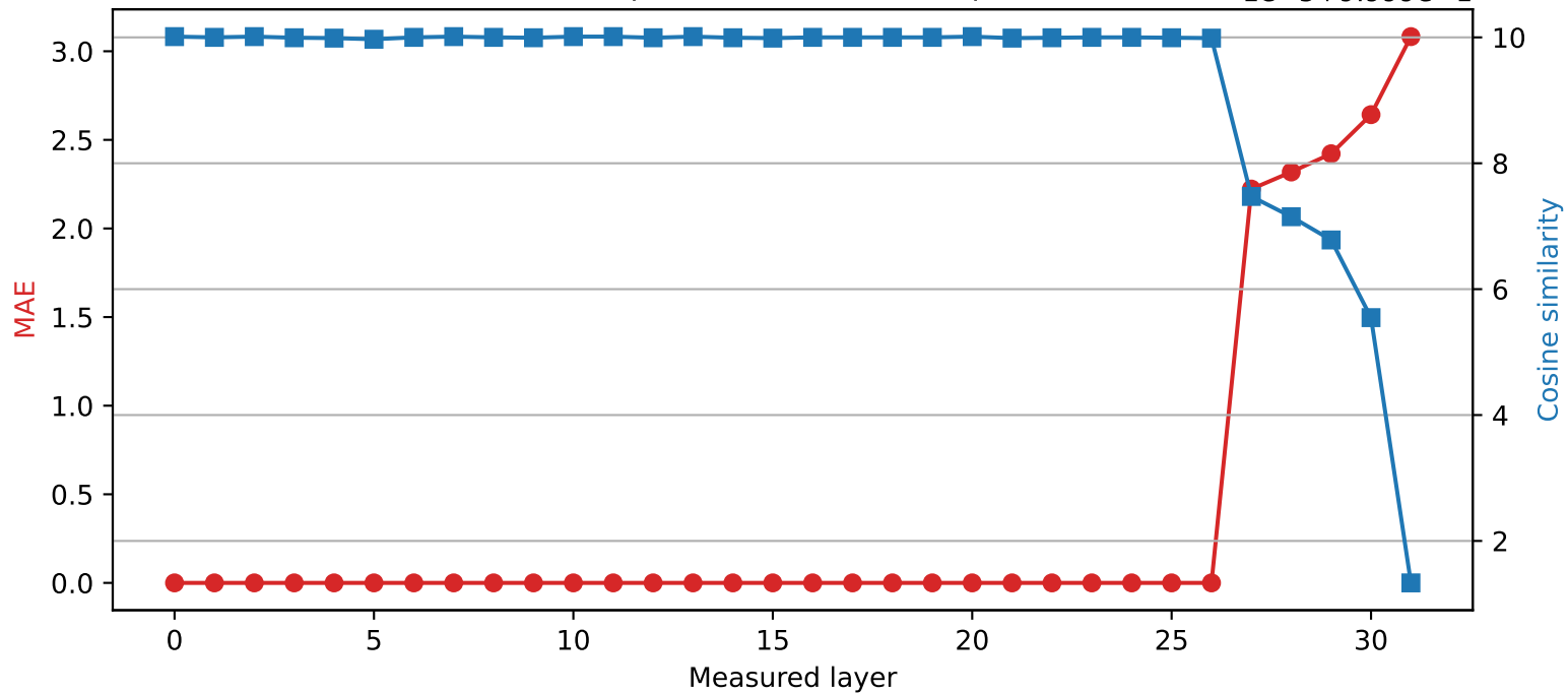
SmolLM2-360M | Quantized layer 26 | float16 \rightarrow int4 1e-5+9.999e-1
